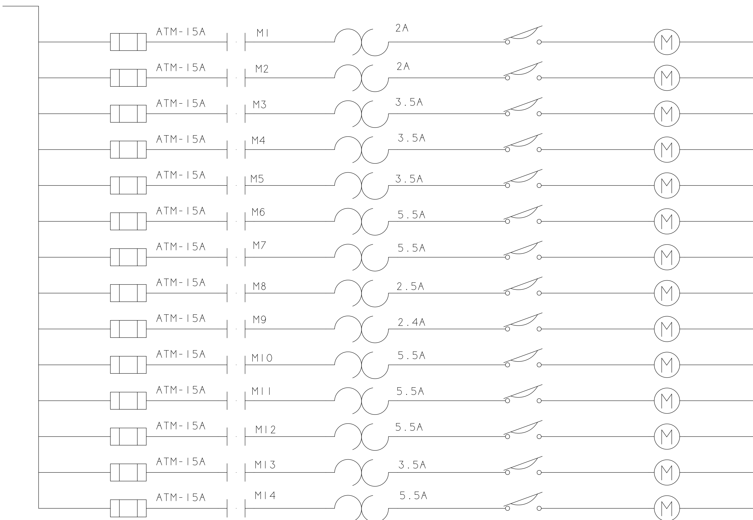
PANEL NH13 1.3.5
